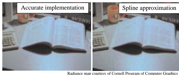
Figure 14: Compare the spline based local operator (right) with the more accurate local operator (left). The spline approach exhibits some blocky artifacts on the table, although this is masked in the rest of the image.
