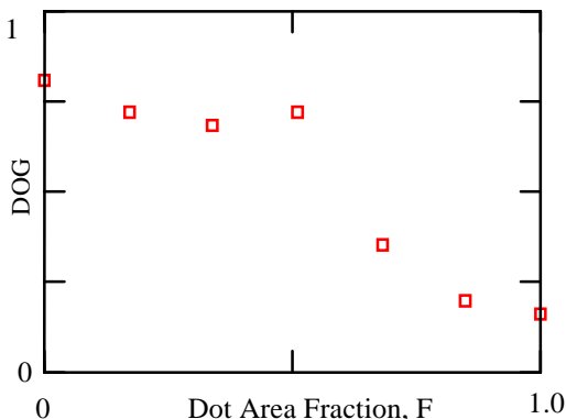
Figure 12. Distinctness of gloss versus dot area fraction for the ink jet samples of Figure 9.
