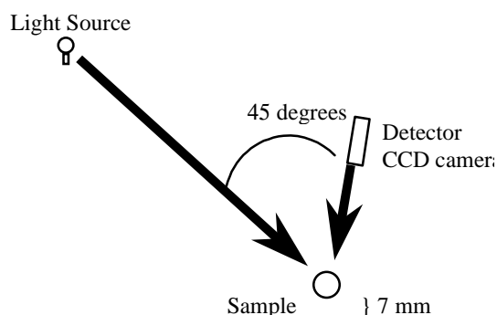
Figure 2. Configuration for the micro-goniophotometer.
