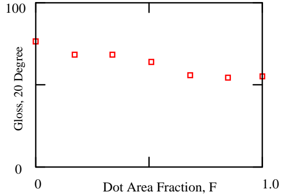
Figure 9. Gloss versus dot area fraction for a clustered dot halftone printed by thermal ink jet with black ink.
