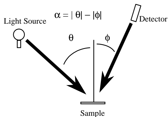
Figure 1. Typical configuration for a goniophotometer.
