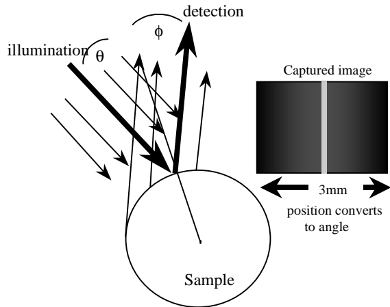
Figure 3. Detail of the cylindrical sample illustrating the relationship between lateral position in the captured image and the goniophotometric angle.
