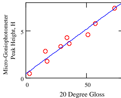
Figure 5. Correlation between the height of the gloss peak and independently measured values for 20 degree gloss.
