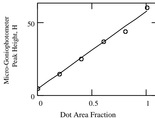
Figure 6. Gloss as a function of dot area fraction for a halftone image made by a phase change ink jet system.
