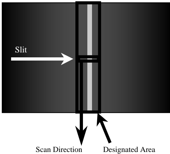
Figure 7. Illustration of spatial scan across the gloss band in the micro-goniophotometer.
