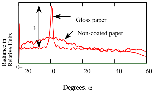
Figure 4. Typical goniophotometric scans from the instrument in Figure 3 for a plain paper and a gloss coated paper.
