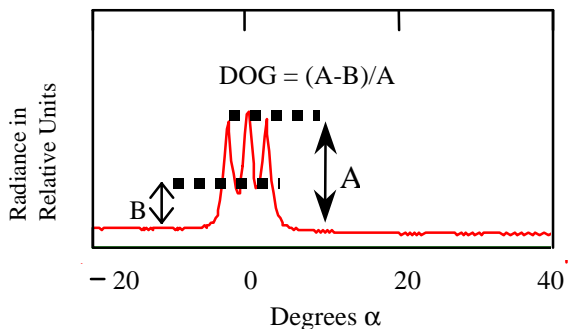
Figure 11. Gloss tri-bar pattern for measurement of the distinctness of gloss.
