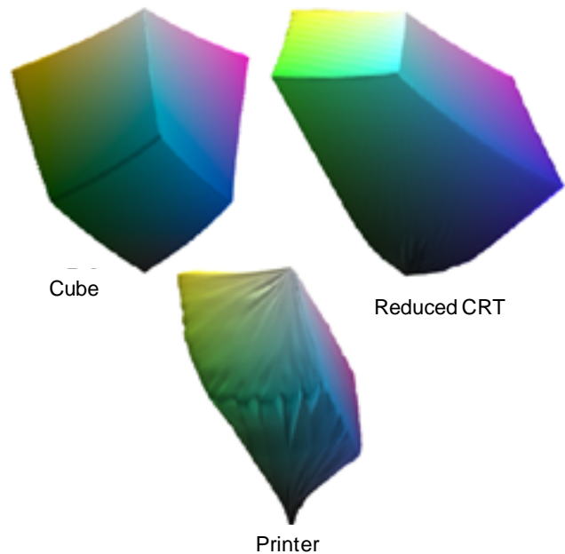
Figure 1. Destination gamuts
