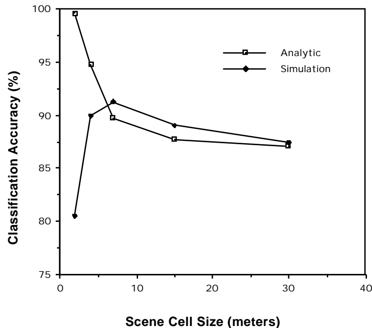
Figure 4.25 Classification Accuracy vs. Ground Size of Scene Cells.
