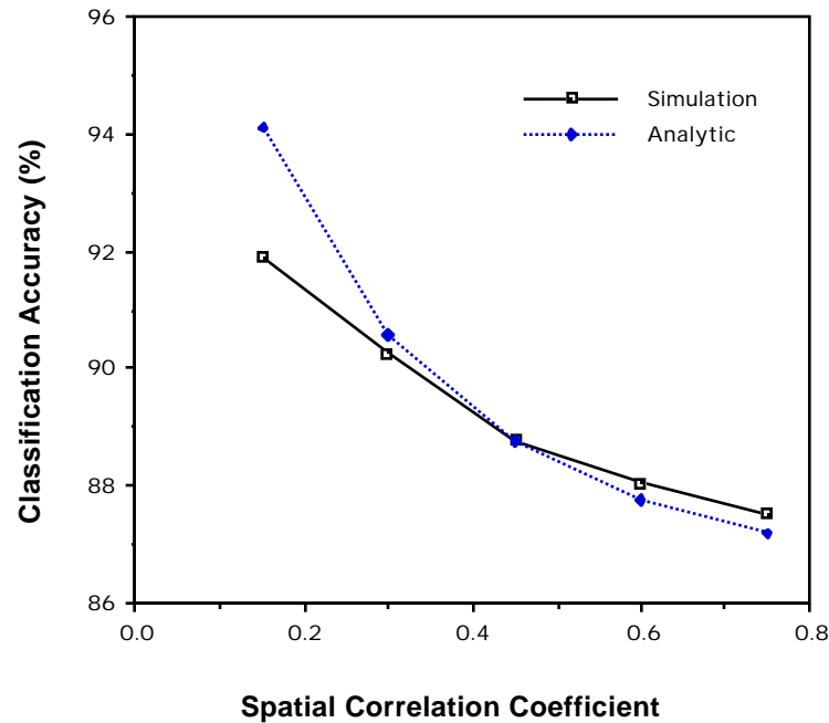
Figure 4.24 Classification Accuracy vs. Scene Spatial Correlation Coefficient.
