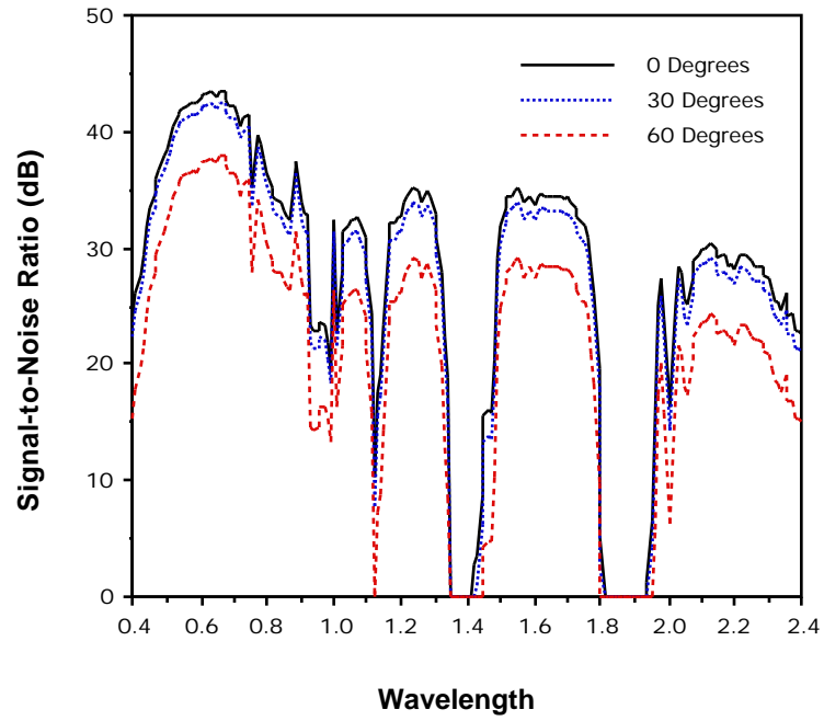
Figure 4.7 SNR for Varying Solar Angles.
