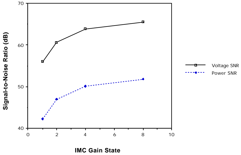
Figure 4.42 Effect of IMC Gain State on SNR.
