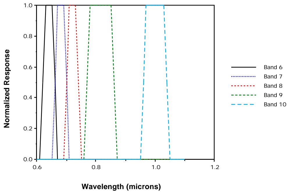
Figure D.2 MMS Spectral Response Bands 6 through 10.
