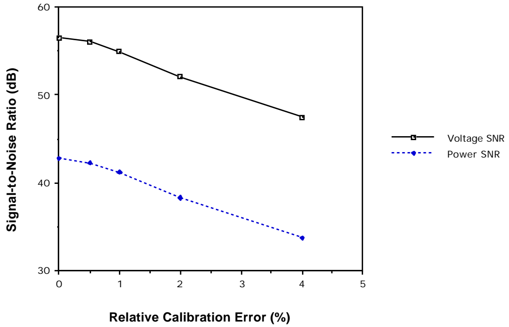
Figure 4.46 Effect of Relative Calibration Error on SNR.
