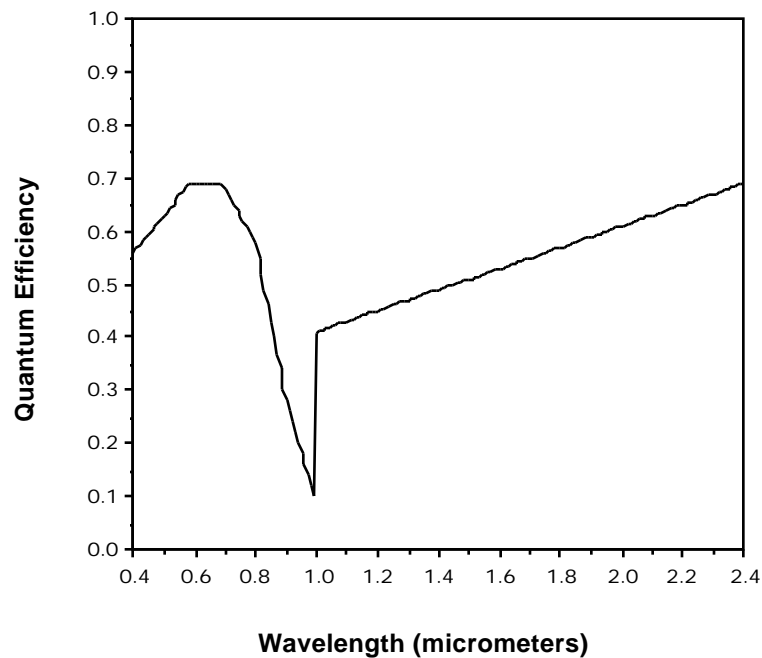
Figure 2.27 Spectral Quantum Efficiency.
