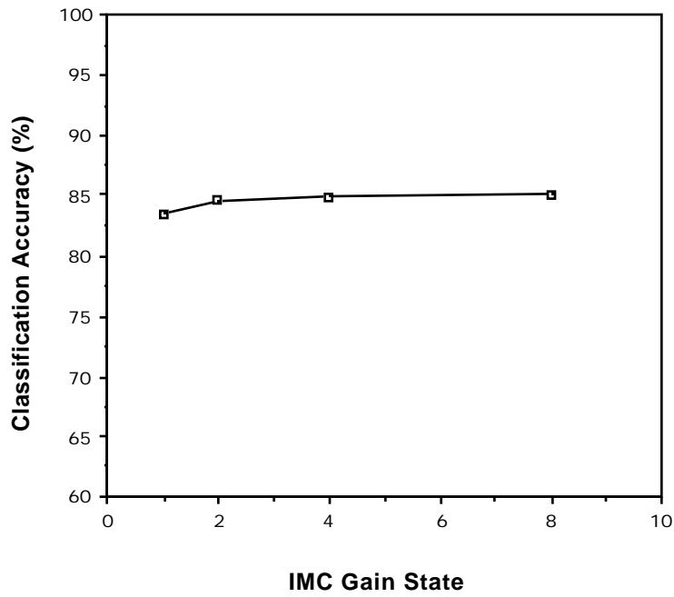
Figure 4.43 Effect of IMC Gain State on Classification Accuracy.
