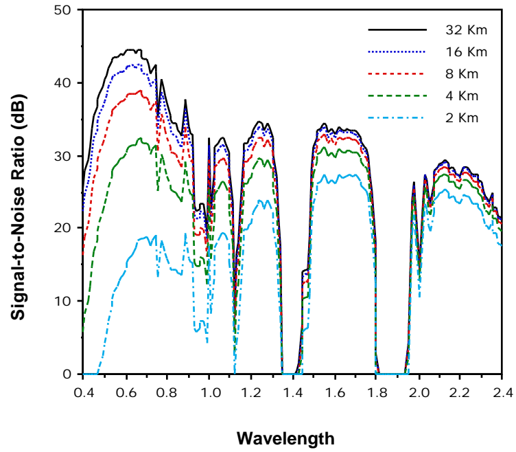
Figure 4.5 SNR for Varying Meteorological Ranges.
