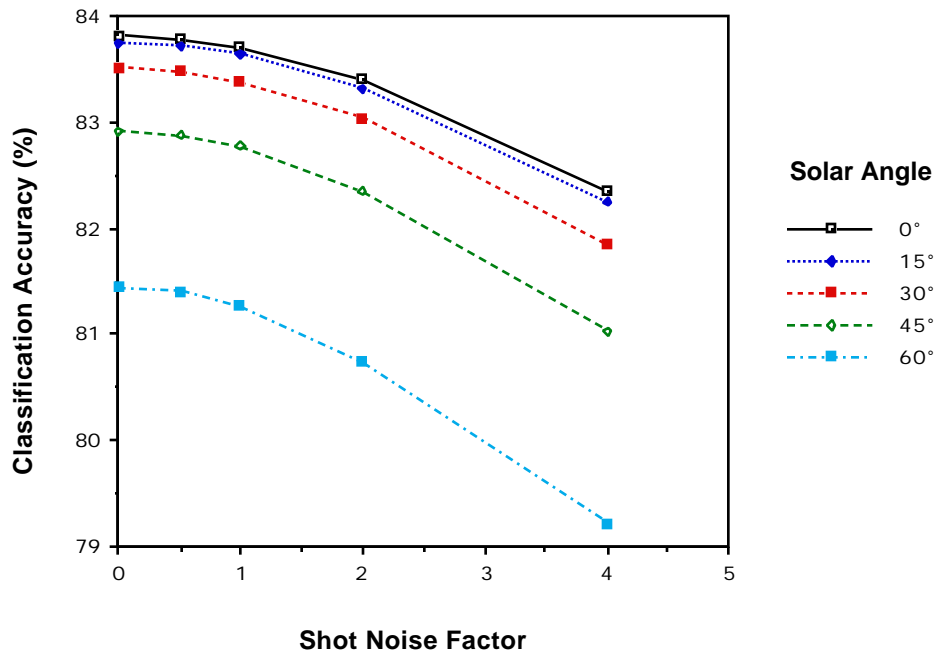
Figure 4.63 Effect of Solar Angle and Shot Noise.
