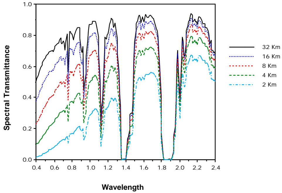
Figure 2.15 Effect of Meteorological Range on Spectral Transmittance.
