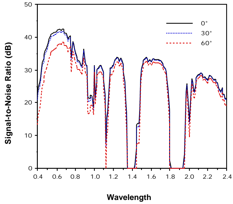
Figure 4.9 SNR for Varying View Angles.
