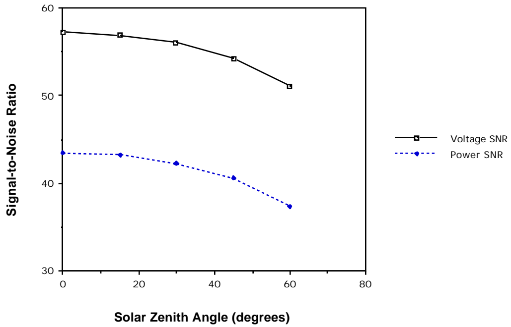
Figure 4.32 Effect of Solar Zenith Angle on SNR.
