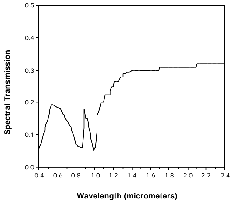
Figure 2.25 Spectral Transmittance of Optics.
