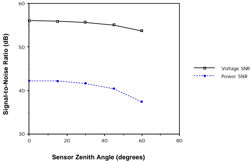
Figure 4.34 Effect of Sensor Zenith Angle on SNR.
