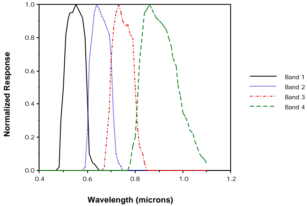
Figure D.3 MSS Spectral Response.
