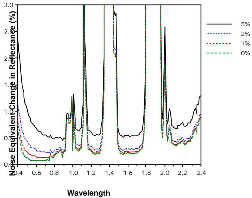
Figure 4.22 NE for Various Levels of Relative Calibration Error.
