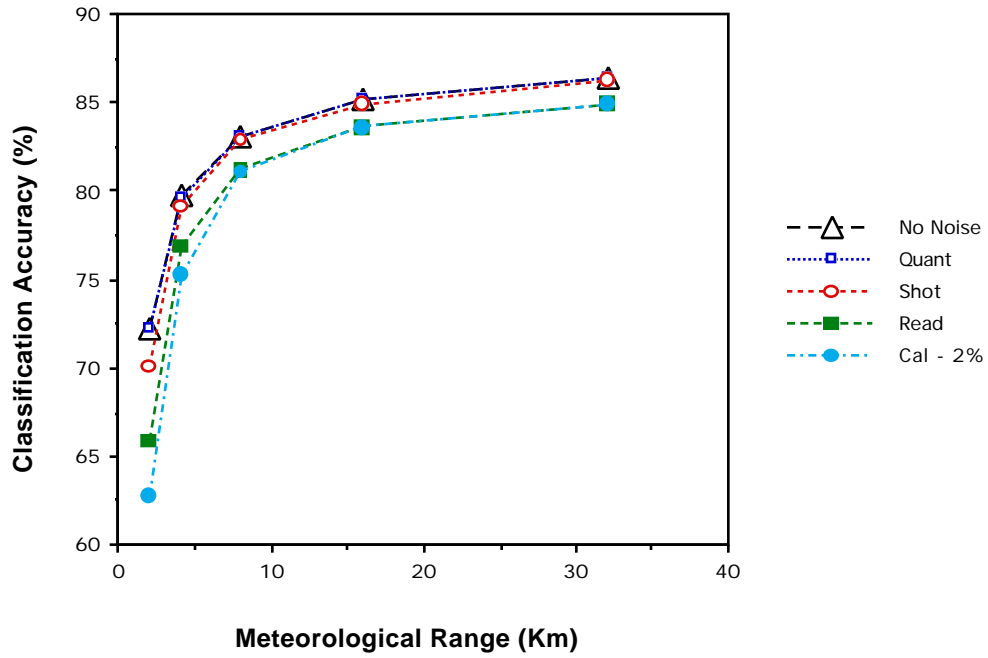
Figure 4.62 Effect of Meteorological Range and Various Noise Sources Alone.
