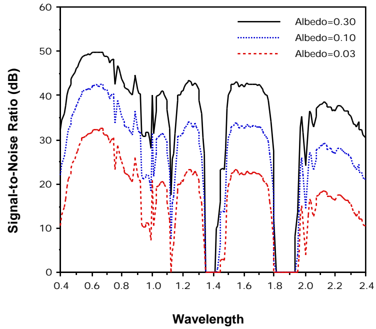
Figure 4.11 SNR for Various Surface Albedoes.
