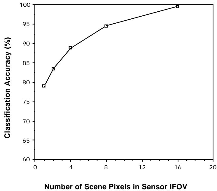
Figure 4.37 Effect of Number of Scene Cells Within Sensor IFOV on Classification Accuracy.
