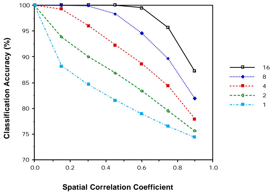
Figure 4.57 Effect of IFOV Size (in Scene Cells) and Spatial Correlation Coefficient.
