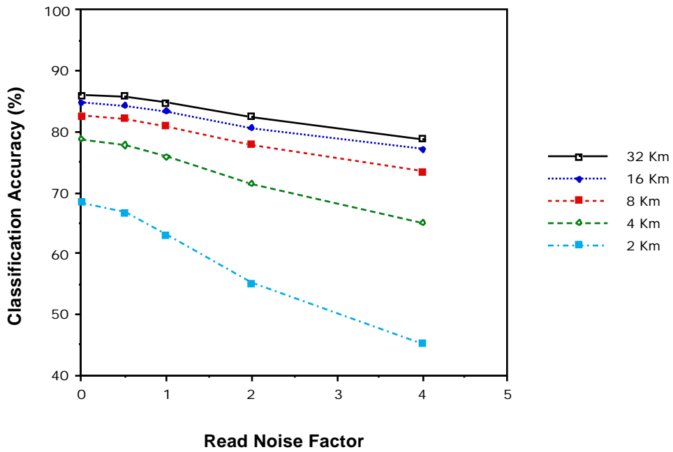
Figure 4.59 Effect of Meteorological Range and Read Noise.
