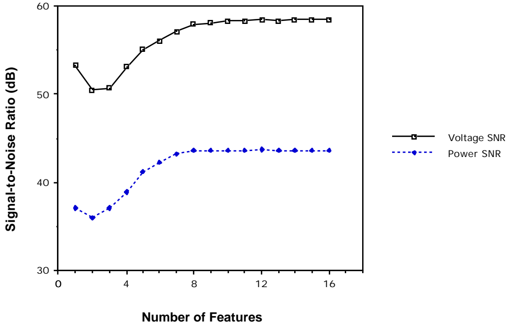
Figure 4.50 Effect of Number of Processing Features on SNR.
