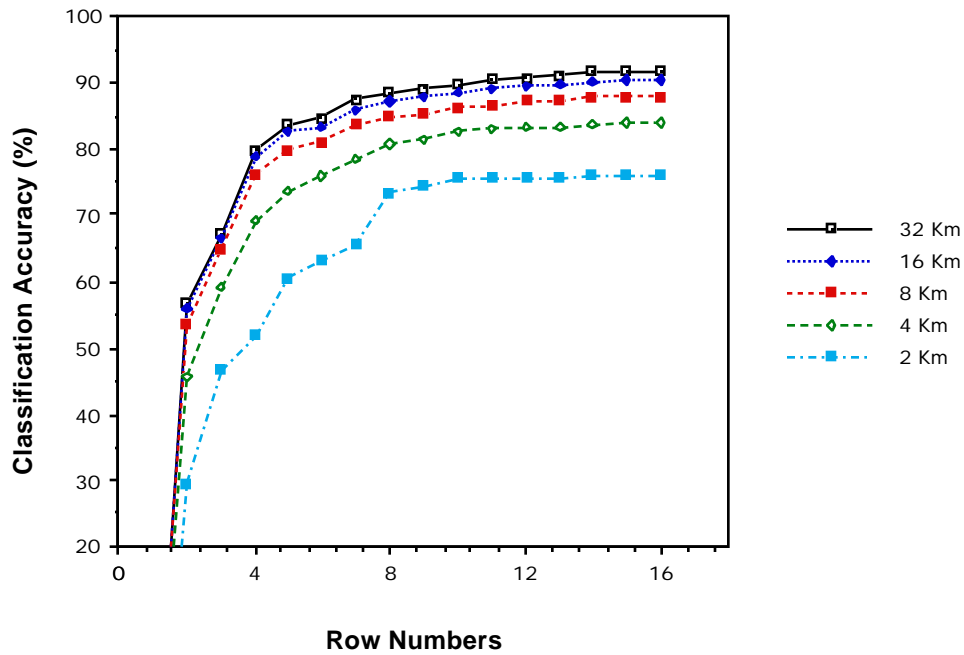
Figure 4.67 Effect of Meteorological Range and Number of Features.
