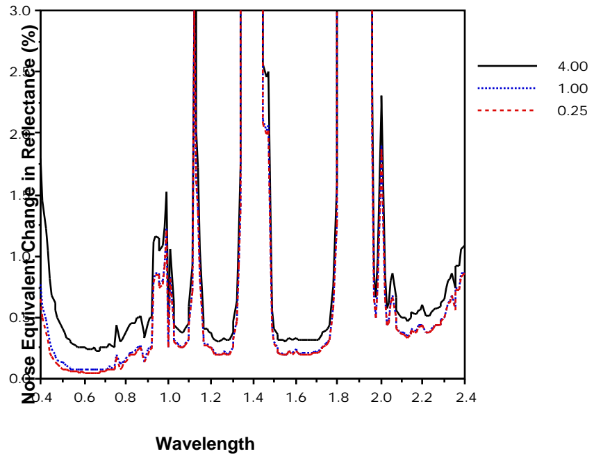
Figure 4.14 NE for Varying Factors of Shot Noise.
