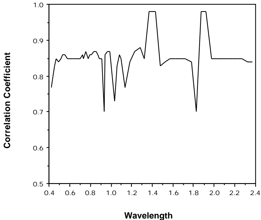
Figure 2.4 Correlation Coefficients of Winter Wheat Field.
