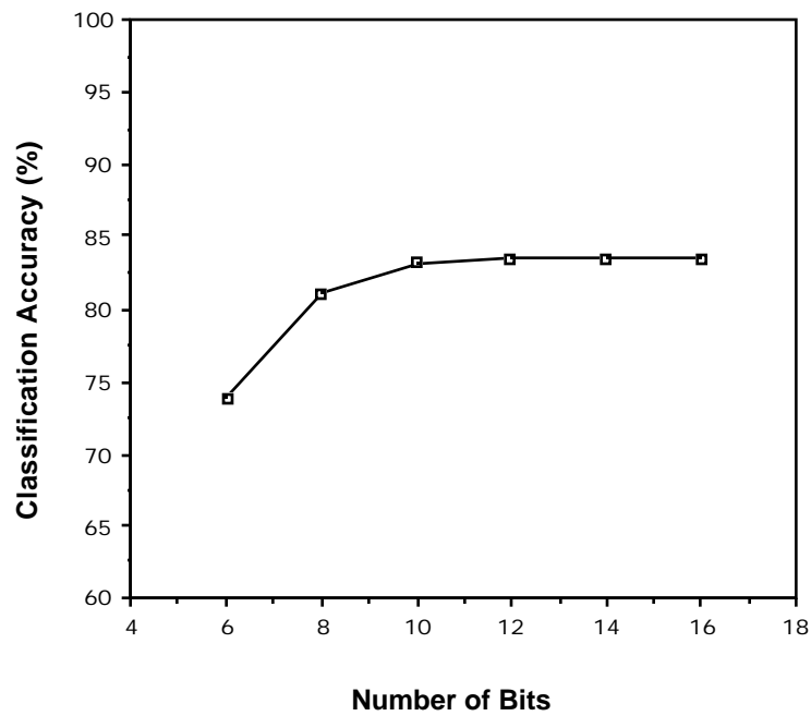
Figure 4.45 Effect of Radiometric Resolution on Classification Accuracy.
