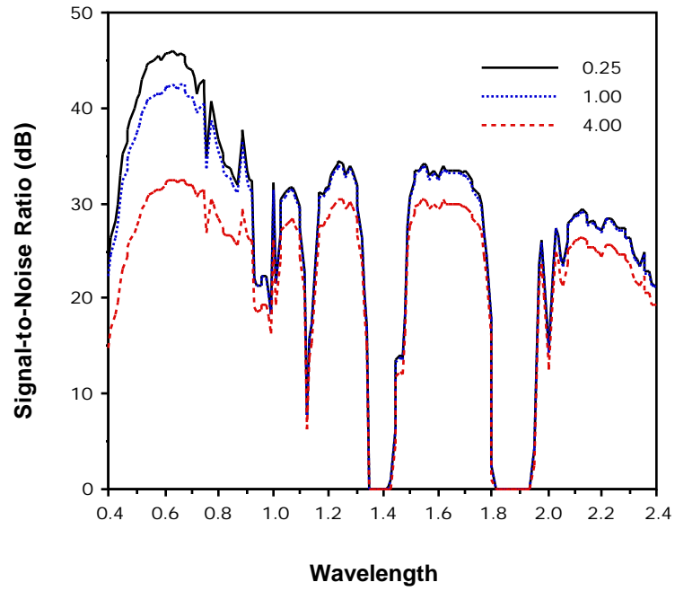
Figure 4.13 SNR for Varying Factors of Shot Noise.
