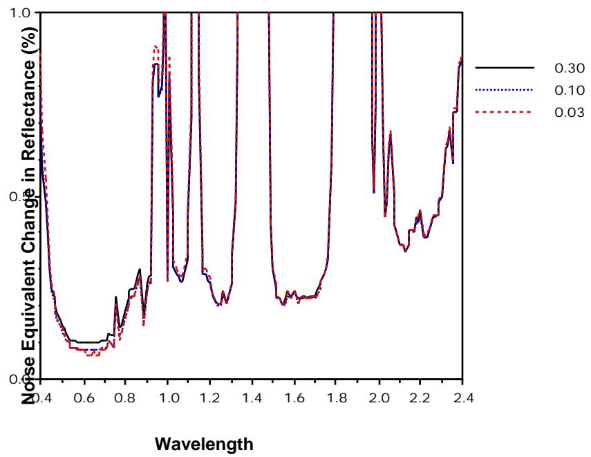
Figure 4.12 NE for Various Albedoes.
