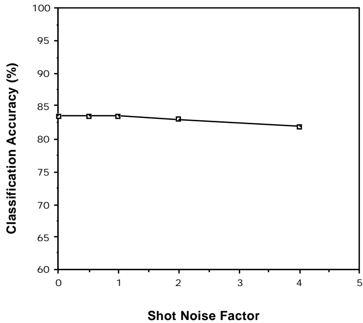
Figure 4.39 Effect of Shot Noise (Nominal = 1.0) on Classification Accuracy.
