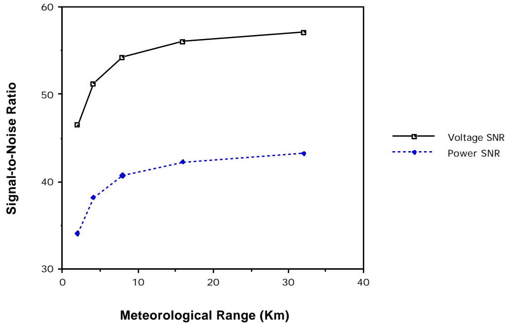
Figure 4.30 Effect of Meteorological Range on SNR.
