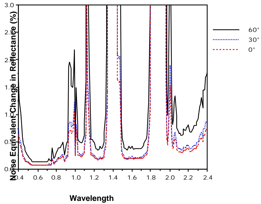
Figure 4.8 NE for Varying Solar Angles.
