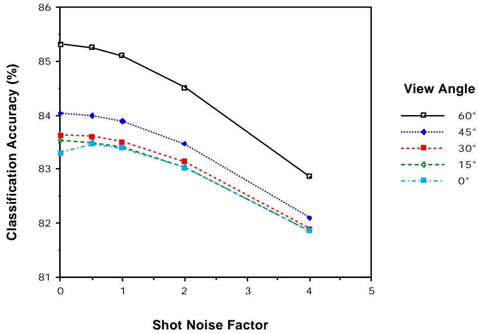
Figure 4.64 Effect of View Angle and Shot Noise.
