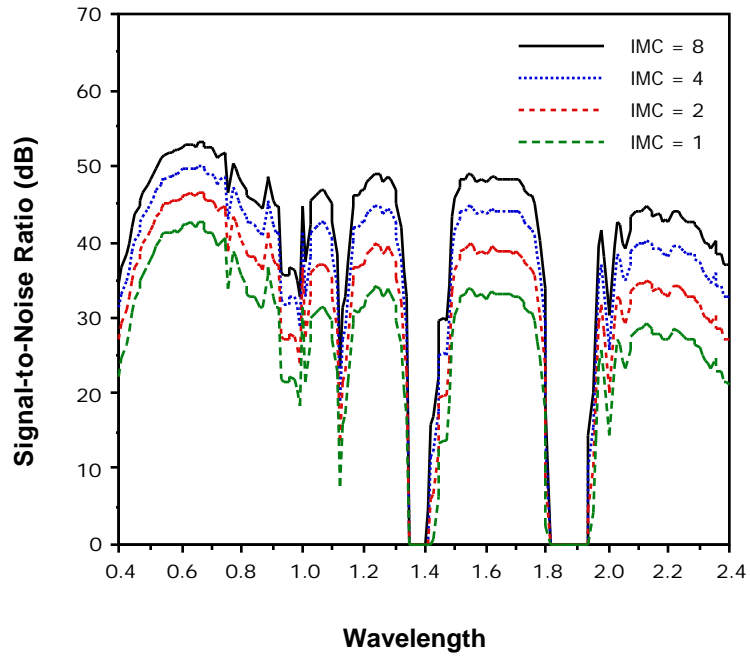
Figure 4.19 SNR for Various IMC Gain Settings.
