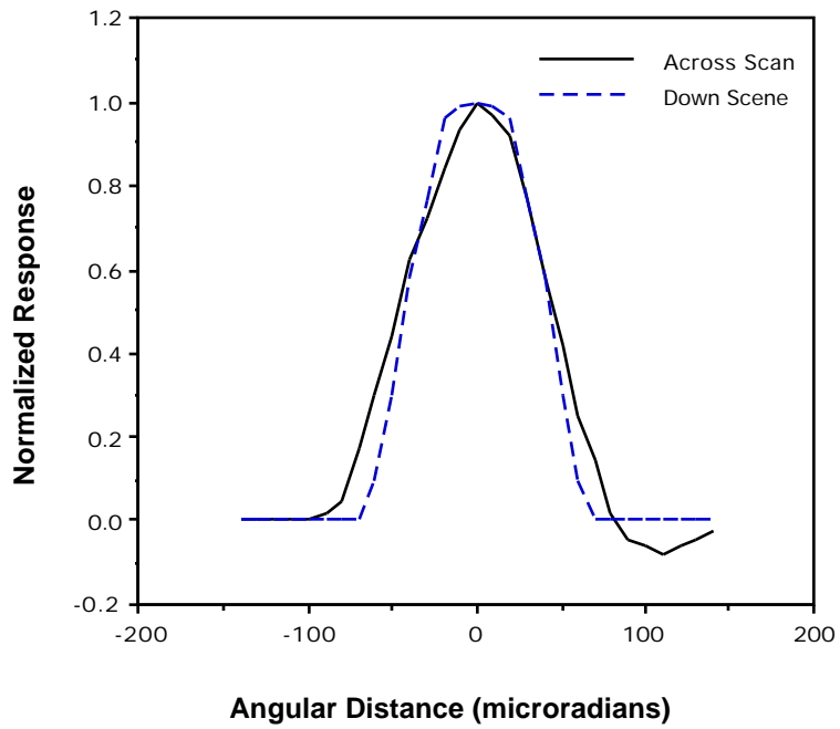
Figure D.4 MSS Spatial Response.
