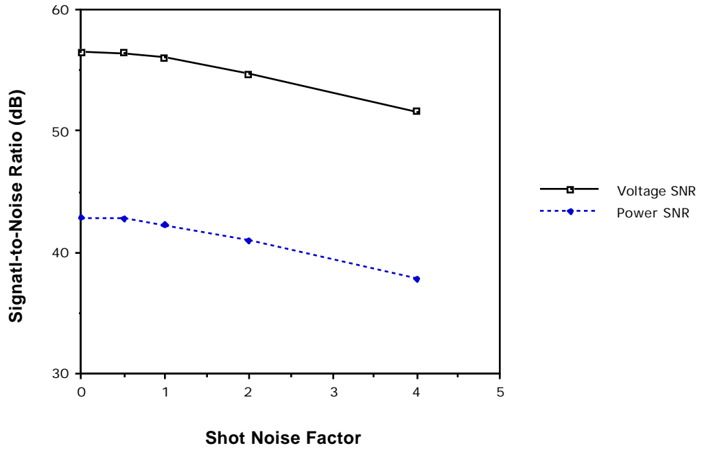
Figure 4.38 Effect of Shot Noise (Nominal = 1.0) on SNR.
