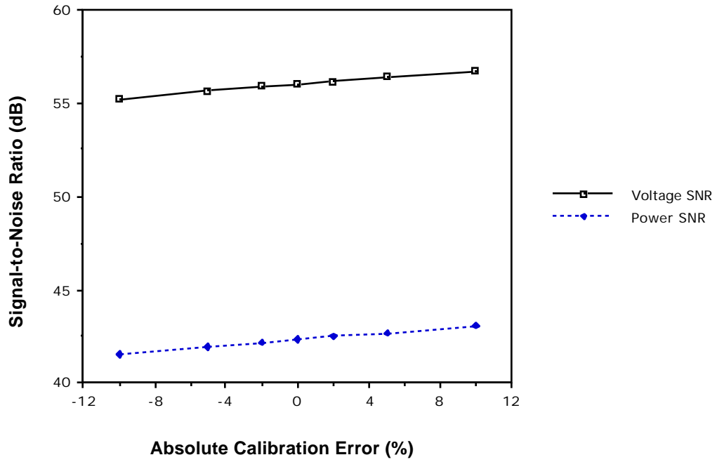
Figure 4.48 Effect of Absolute Radiometric Error on SNR.
