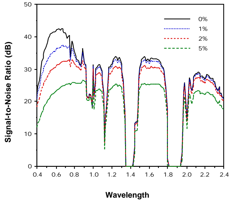
Figure 4.21 SNR for Various Levels of Relative Calibration Error.
