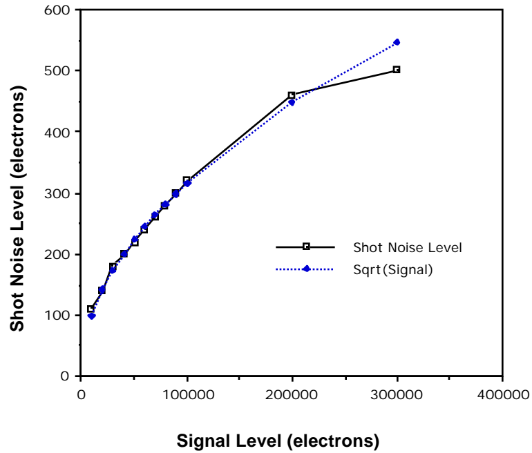
Figure 2.28 Shot Noise vs. Signal Level.
