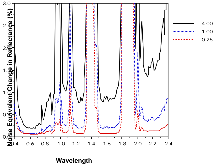
Figure 4.16 NE for Varying Factors of Read Noise.
