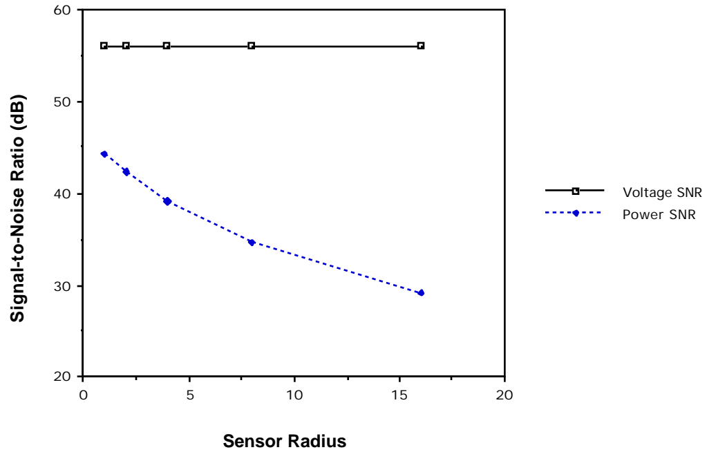
Figure 4.36 Effect of Number of Scene Cells Within Sensor IFOV on SNR.
