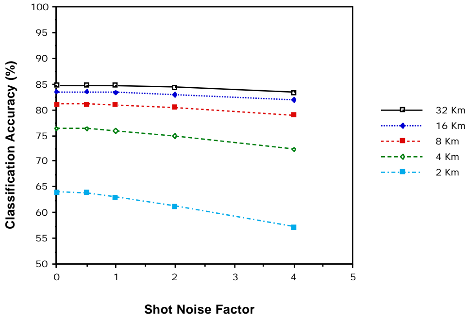
Figure 4.58 Effect of Meteorological Range and Shot Noise.
