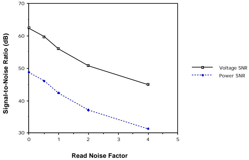
Figure 4.40 Effect of Read Noise (Nominal = 1.0) on SNR.
