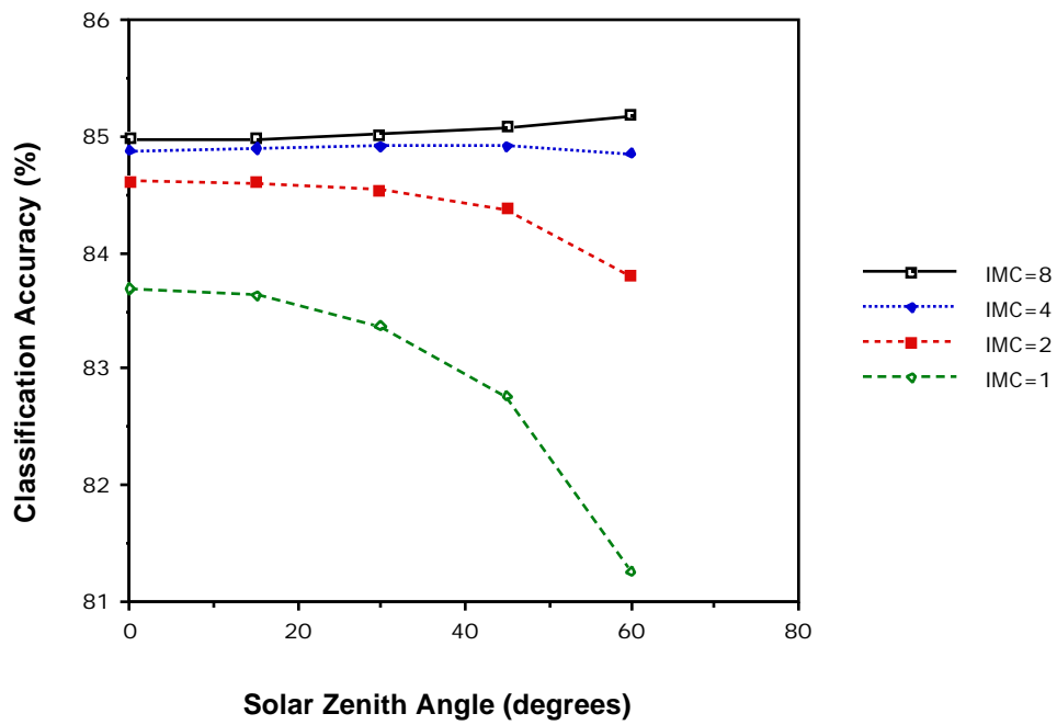
Figure 4.65 Effect of Solar Angle and IMC Gain State.
