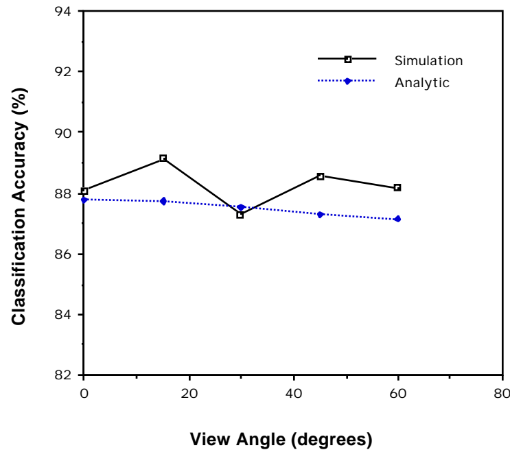
Figure 4.26 Classification Accuracy vs. Sensor View Angle.
