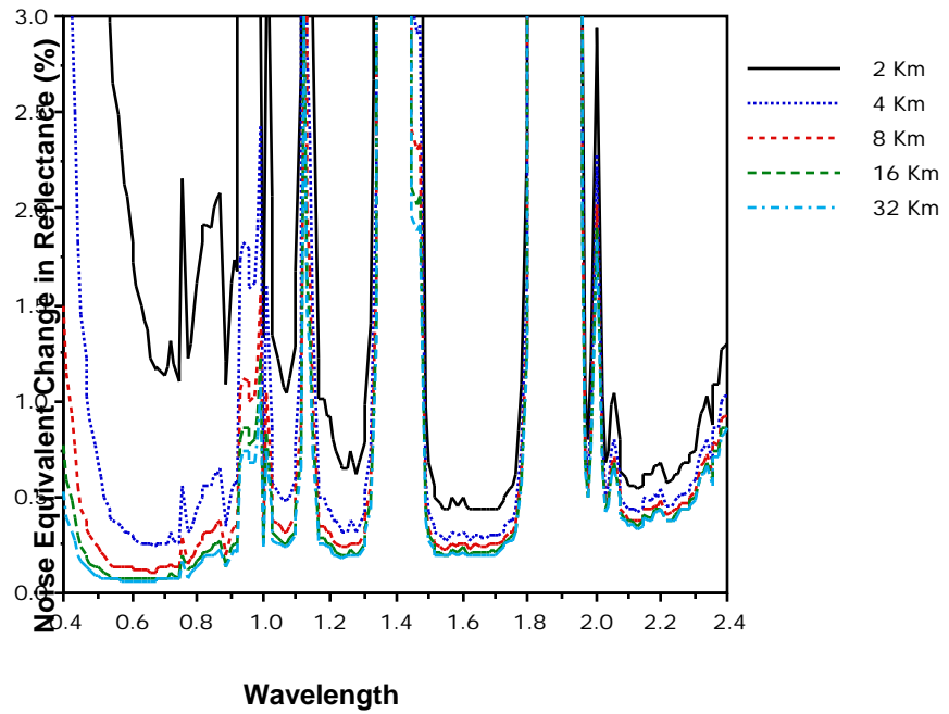
Figure 4.6 NE for Varying Meteorological Ranges.
