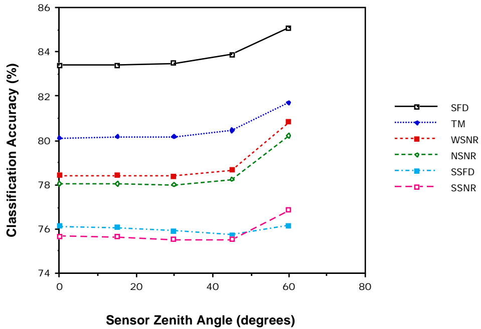
Figure 4.74 Feature Set Performance vs. View Angle.
