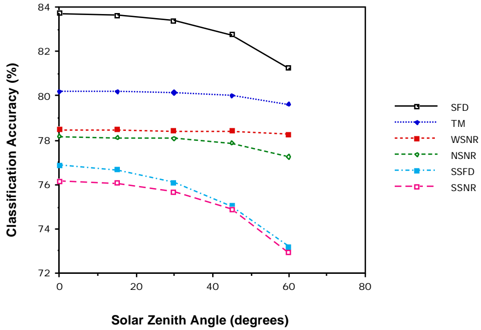
Figure 4.73 Feature Set Performance vs. Solar Angle.
