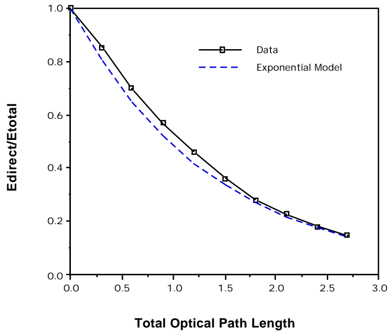
Figure 2.8 Ratio of Direct to Total Irradiance vs. Total Optical Path Length.
