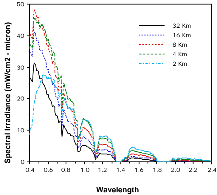
Figure 2.13 Effect of Meteorological Range on Diffuse Solar Spectral Irradiance.
