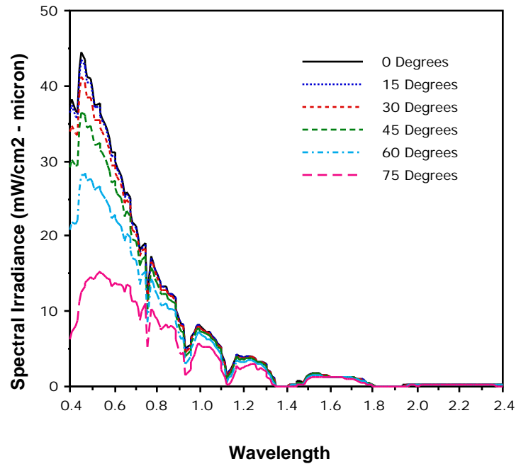
Figure 2.14 Effect of Solar Zenith Angle on Diffuse Solar Spectral Irradiance.
