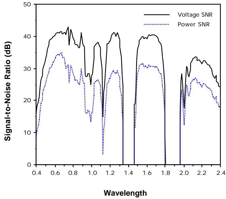
Figure 4.3 Voltage and Power SNR for Typical Reflectance.
