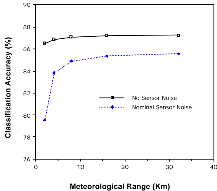
Figure 4.69 Effect of Atmosphere With/Without Noise For Path Radiance Model With No Surface Reflectance Dependence.
