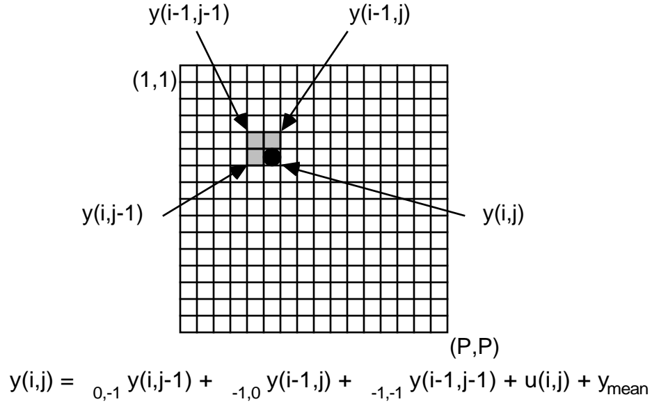
Figure A.1 Quarter-Plane Image AR Model.
