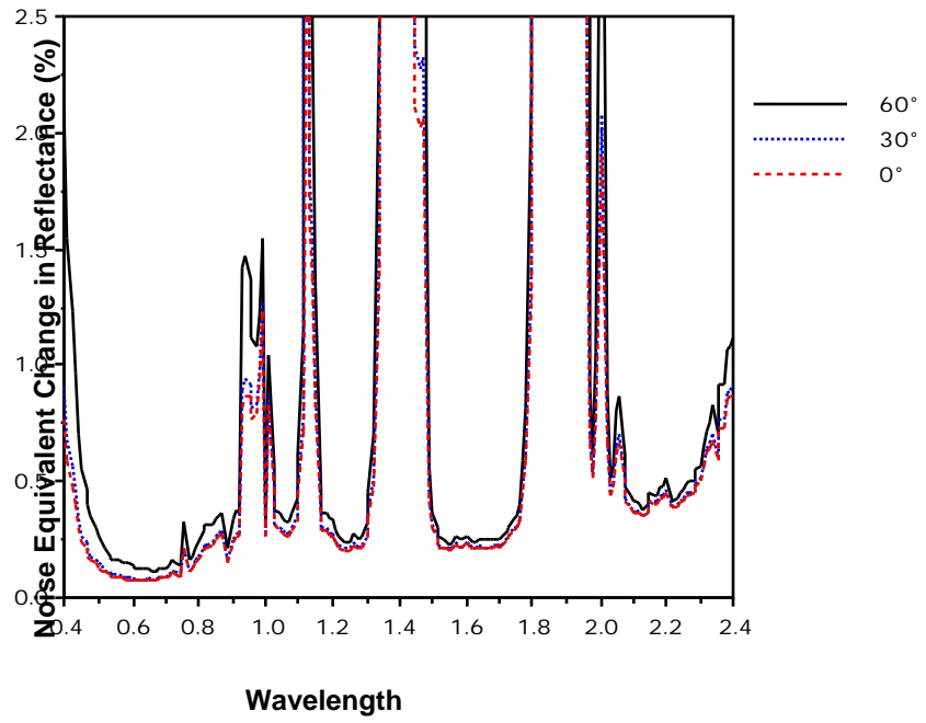
Figure 4.10 NE for Varying View Angles.
