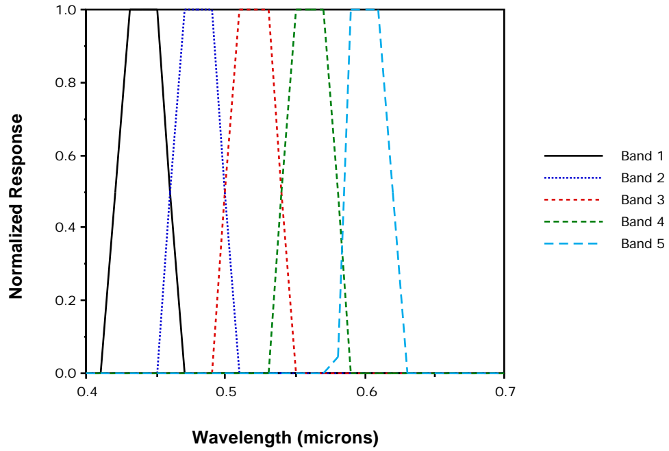
Figure D.1 MMS Spectral Response for Bands 1 though 5.
