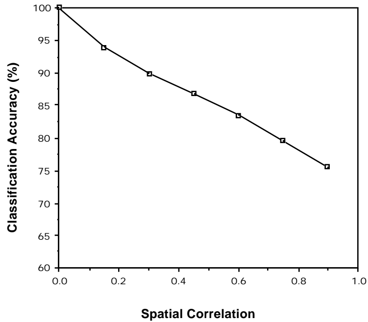
Figure 4.29 Effect of Spatial Correlation ( \rho_x = \rho_y ) on Classification Accuracy.
