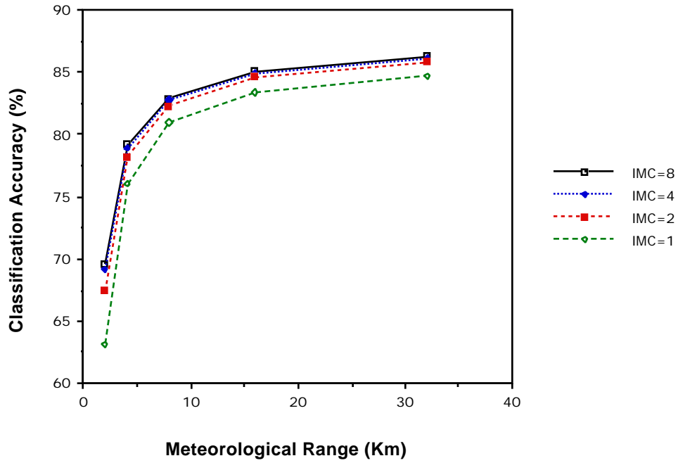
Figure 4.60 Effect of Meteorological Range and IMC.
