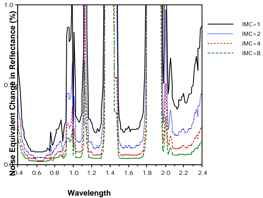
Figure 4.20 NE for Various IMC Gain Settings.
