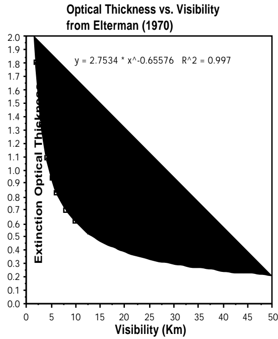
Figure 2.6 Optical Thickness vs. Visibility.
