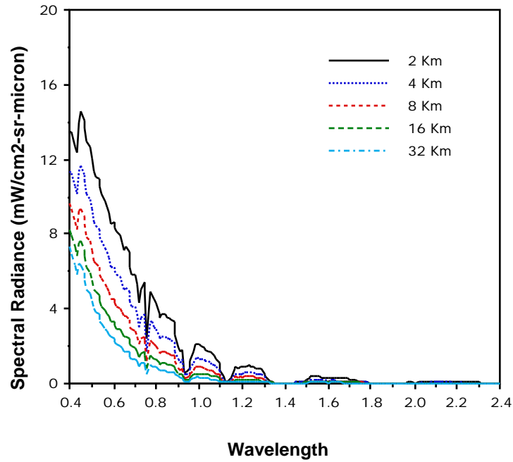
Figure 2.17 Effect of Meteorological Range on Path Spectral Radiance.
