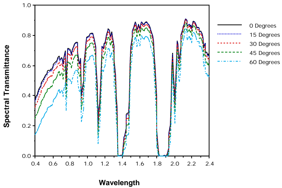
Figure 2.16 Effect of Sensor Zenith Angle on Spectral Transmittance.
