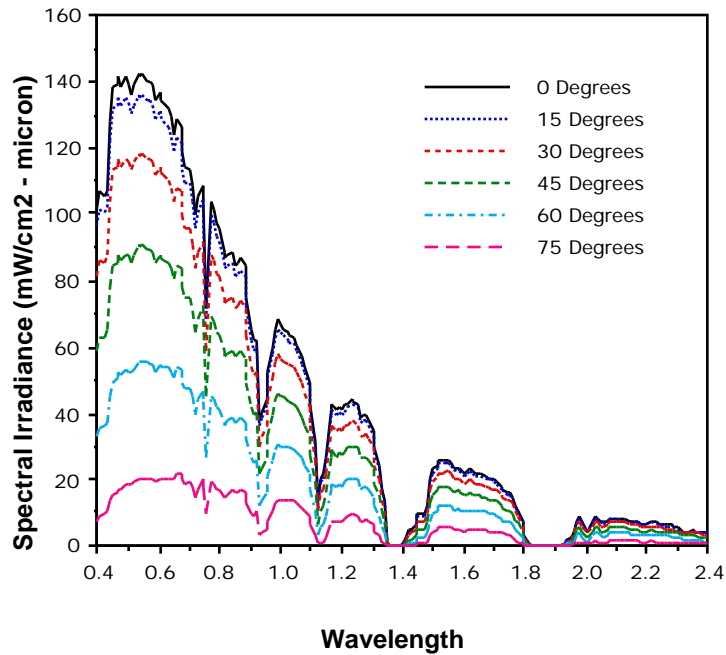
Figure 2.12 Effect of Solar Zenith Angle on Total Solar Spectral Irradiance.
