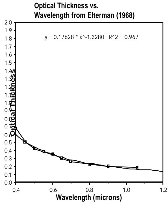
Figure 2.7 Optical Thickness vs. Wavelength.
