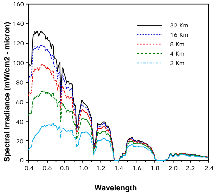
Figure 2.11 Effect of Meteorological Range on Total Solar Spectral Irradiance.
