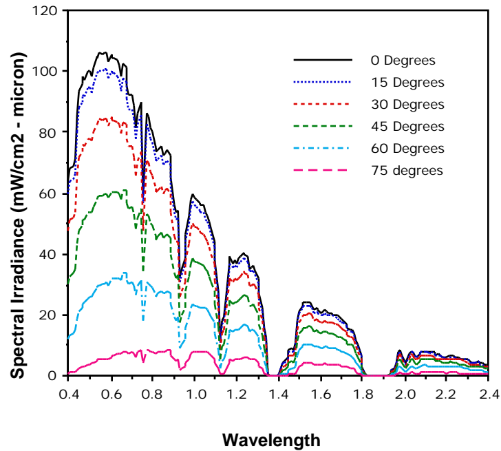
Figure 2.10 Effect of Solar Zenith Angle on Direct Solar Spectral Irradiance.
