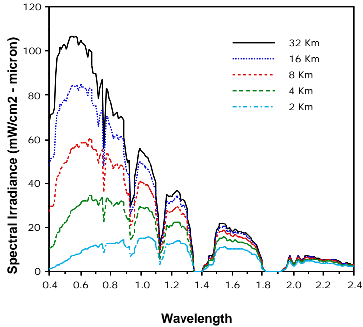
Figure 2.9 Effect of Meteorological Range on Direct Solar Spectral Irradiance.
