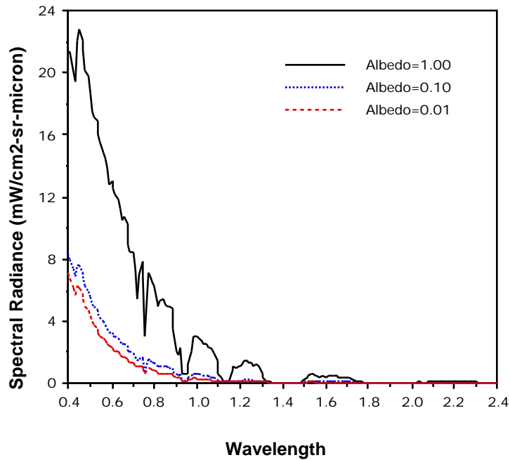
Figure 2.20 Effect of Surface Albedo on Path Spectral Radiance.
