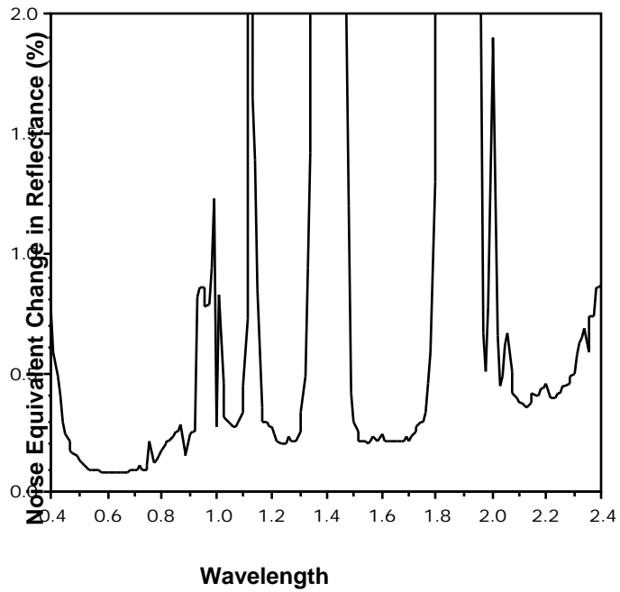
Figure 4.4 NE for Typical Reflectance.
