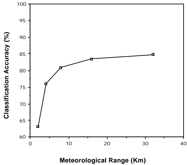
Figure 4.31 Effect of Meteorological Range on Classification Accuracy.
