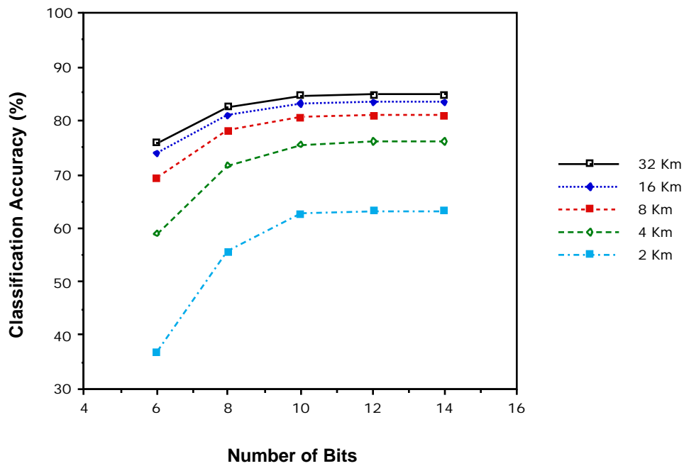
Figure 4.61 Effect of Meteorological Range and Radiometric Resolution.
