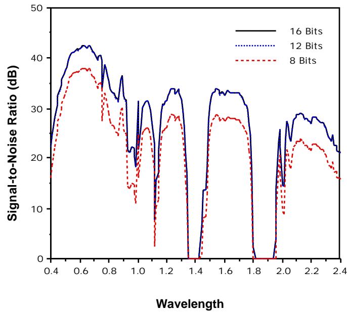
Figure 4.17 SNR for Varying Radiometric Resolution. The SNR for 12 and 16 Bits is Identical.
