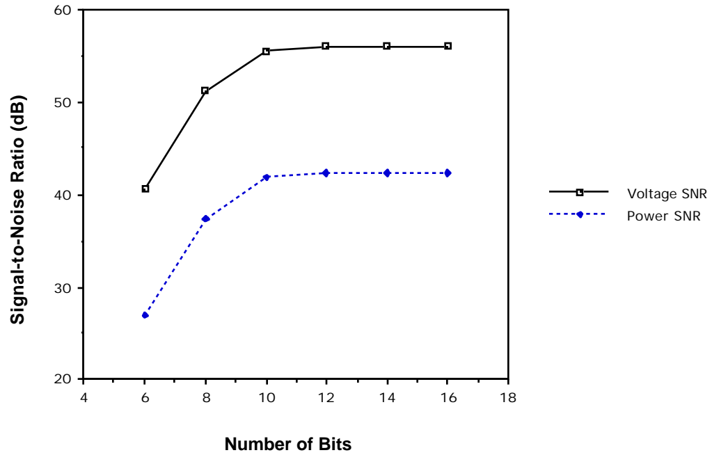
Figure 4.44 Effect of Radiometric Resolution on SNR.
