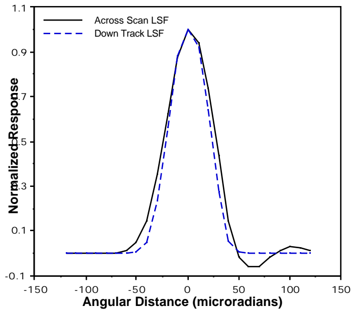
Figure D.6 TM Spatial Response.
