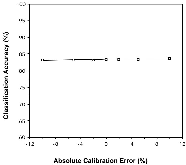
Figure 4.49 Effect of Absolute Radiometric Error on Classification Accuracy.
