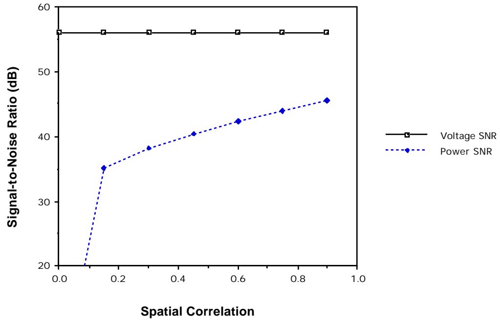
Figure 4.28 Effect of Spatial Correlation ( \rho_x = \rho_y ) on SNR.
