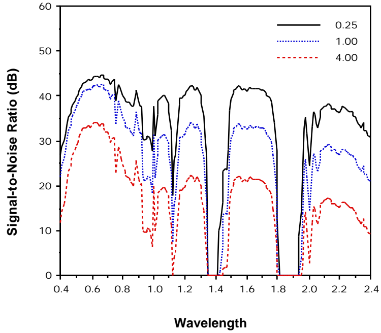
Figure 4.15 SNR for Varying Factors of Read Noise.
