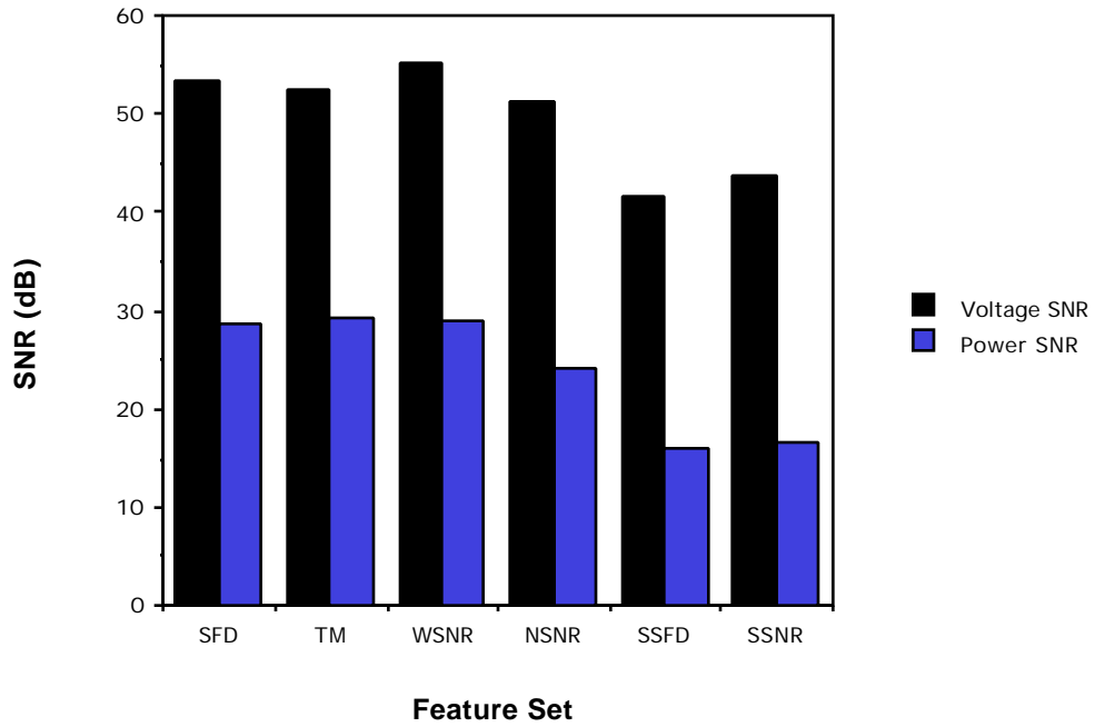
Figure 4.75 SNR for Various Feature Sets and SW Variety Scene.
