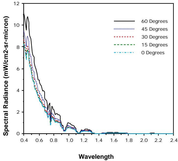
Figure 2.19 Effect of Sensor Zenith Angle on Path Spectral Radiance.
