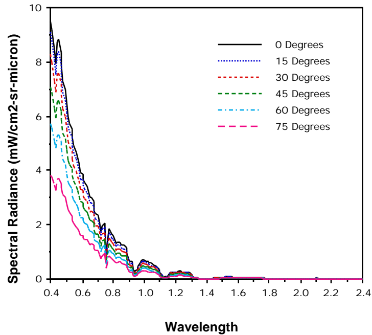
Figure 2.18 Effect of Solar Zenith Angle on Path Spectral Radiance.
