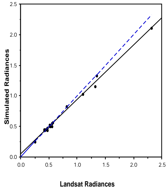
Figure 2.21. Plot of Landsat vs. Simulated Radiances.
