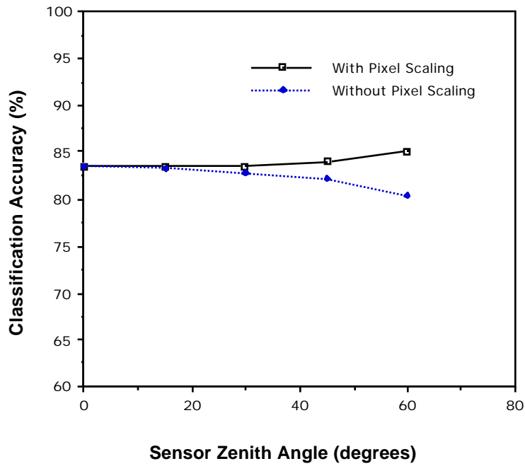
Figure 4.35 Effect of Sensor Zenith Angle on Classification Accuracy.
