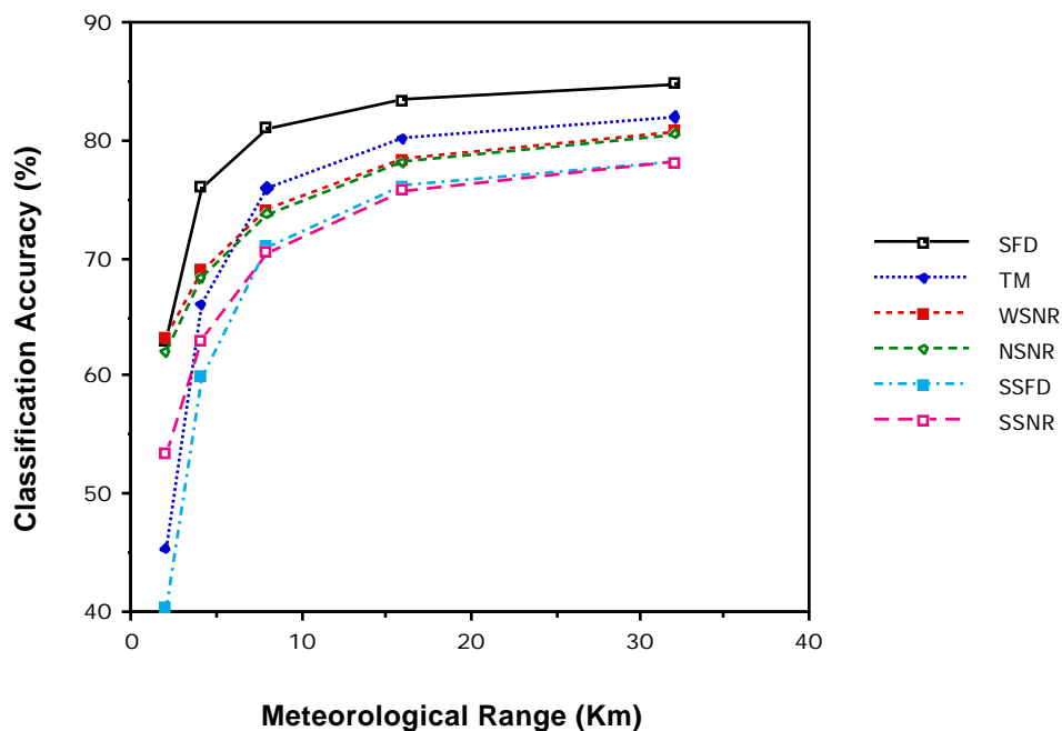
Figure 4.72 Feature Set Performance vs. Meteorological Range.
