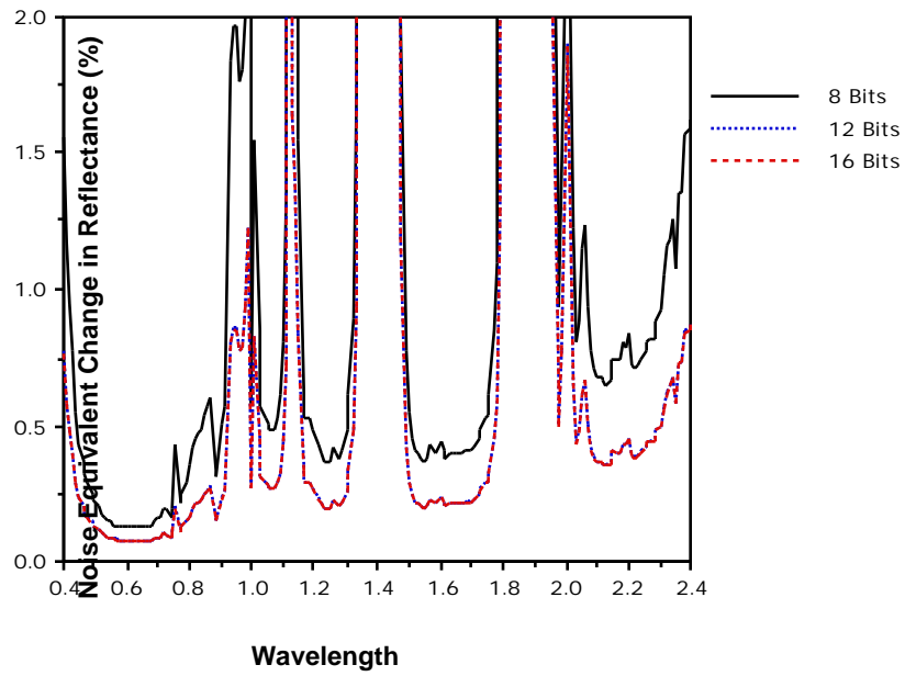
Figure 4.18 NE for Various Radiometric Resolutions. The NE for 12 and 16 Bits is Identical.
