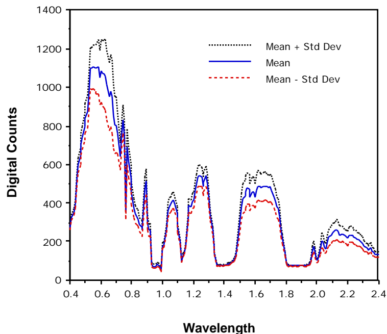
Figure 4.2 Mean and Variation of the Image Vector as Received by HIRIS.
