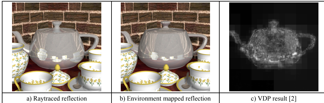
Fig 1. Images rendered with different reflection algorithms and VDP map showing areas of visible difference.
