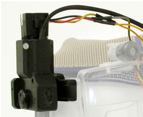
Figure 5a – Close-up of the ASL optics module
