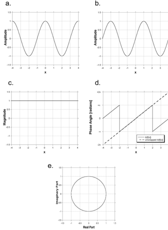
Figure 3: Representations of the complex sinusoidal function f[x] = e^{+2\pi i \xi_0 x} = \cos[2\pi \xi_0 x] + i \sin[2\pi \xi_0 x] as (a) real part; (b) imaginary part; (c) magnitude; (d) phase; and (e) Argand diagram.
