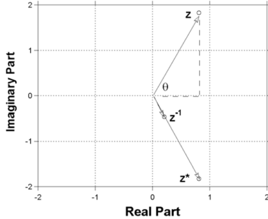
Figure 1: Argand Diagrams of z , z^{-1} , and z^* .
