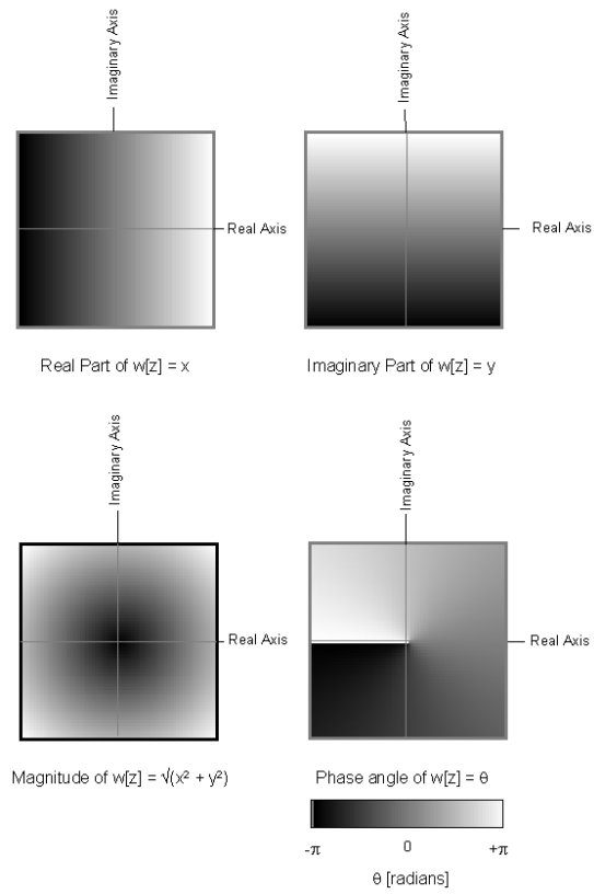
Figure 2: The complex function w[z] = z = x + iy , represented as real-and-imaginary parts and as magnitude-and-phase.
