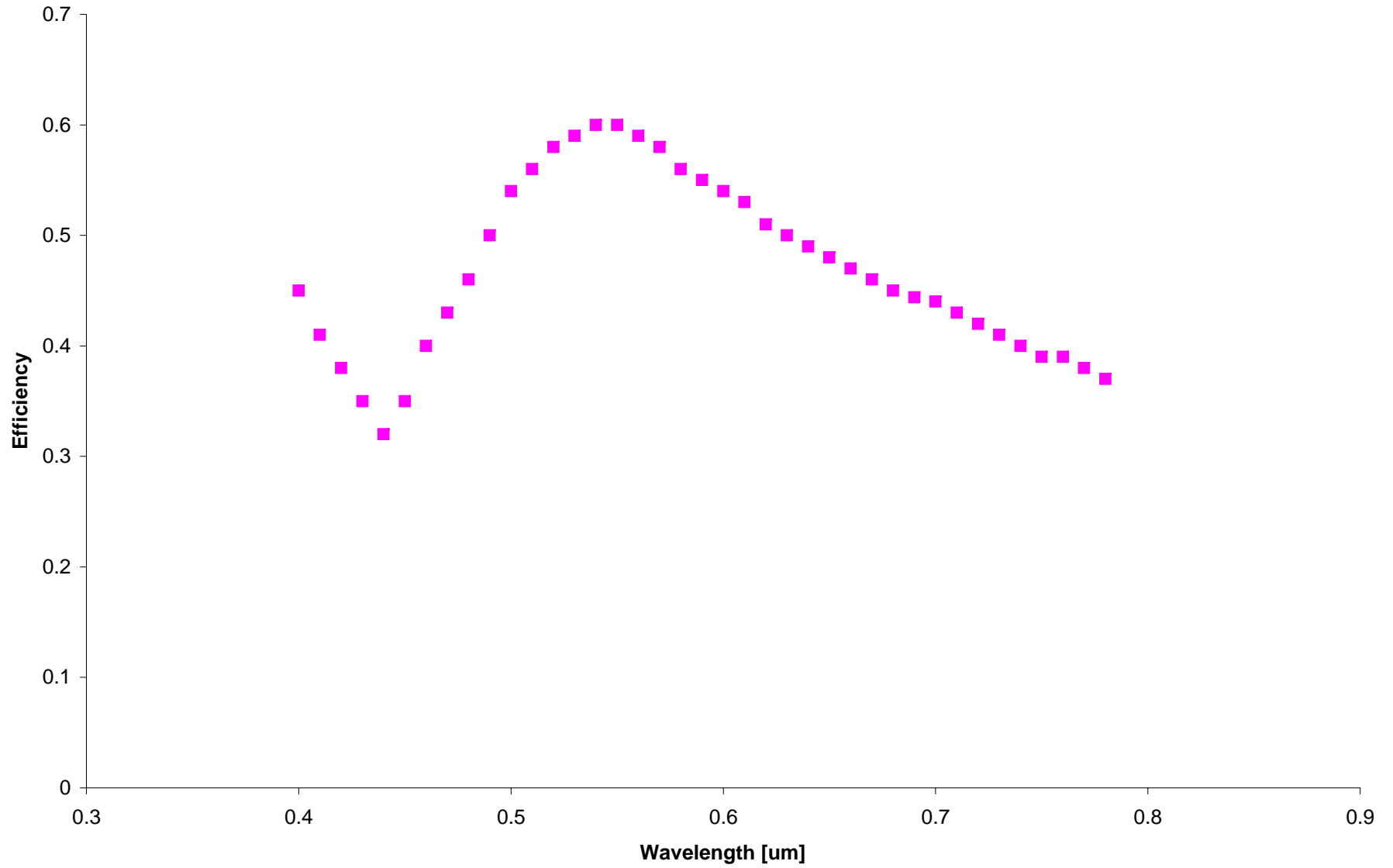
Monochromator Efficiency
