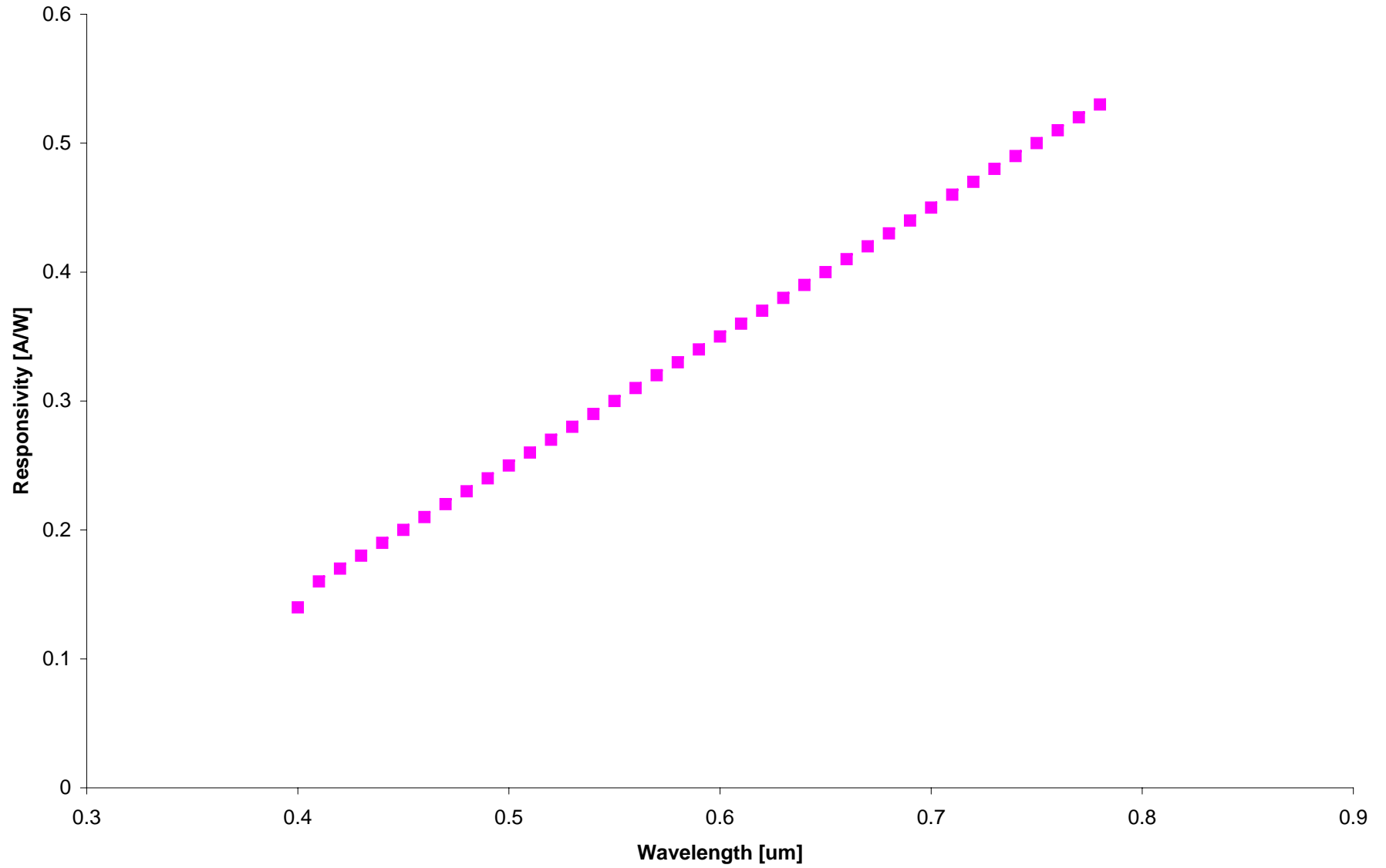
Detector Responsivity
